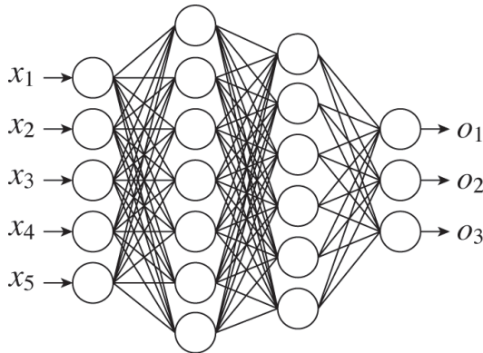
Fig. 1: A neural network structure
